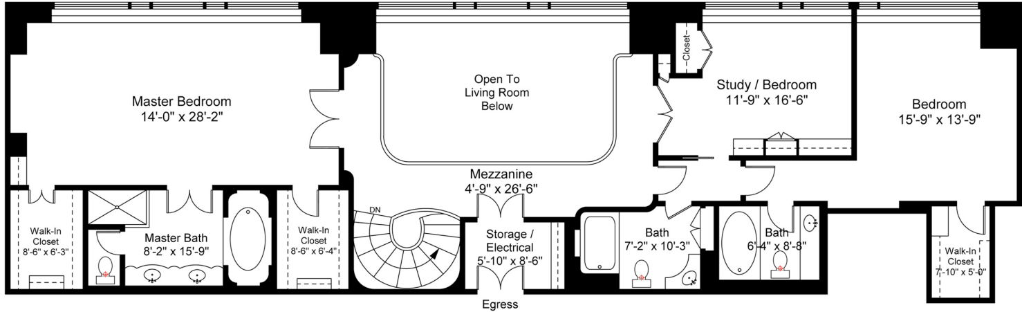
SECOND FLOOR
